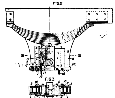
DETAILS OF MARTELL PEDESTAL.
